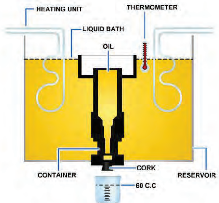
Figure 3-1 — Saybolt viscometer.
