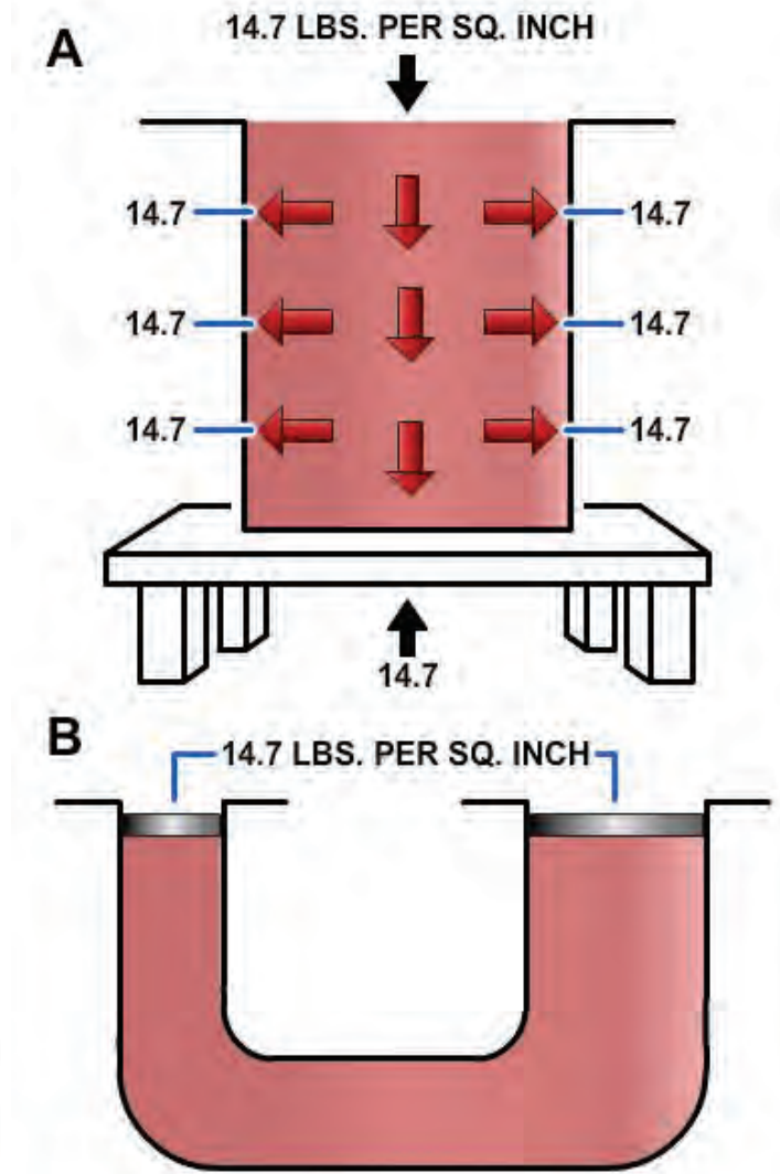
Figure 2-3 — Effects of atmospheric pressure.
