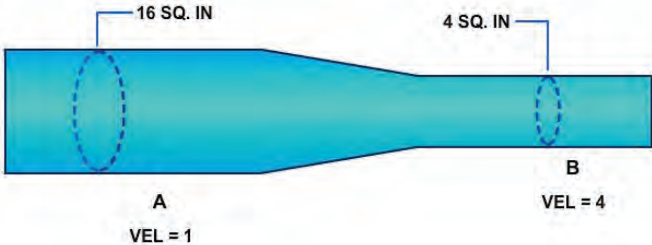
Figure 2-13 — Volume and velocity of flow.
