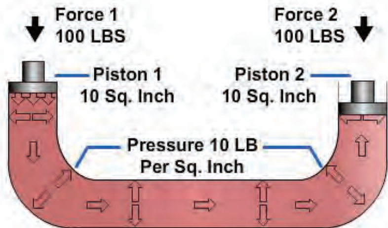
Transmitted Force Through Fluid
